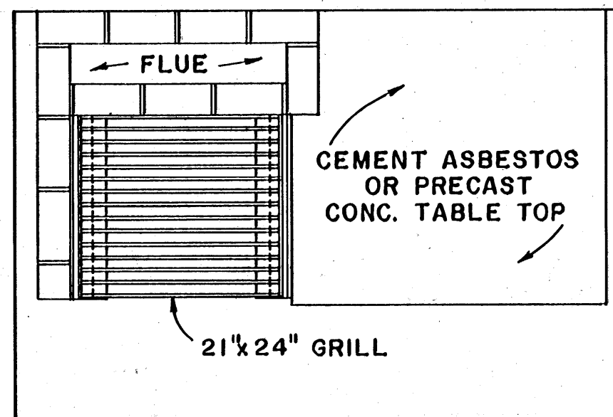
PLAN AT WORKING LEVEL
