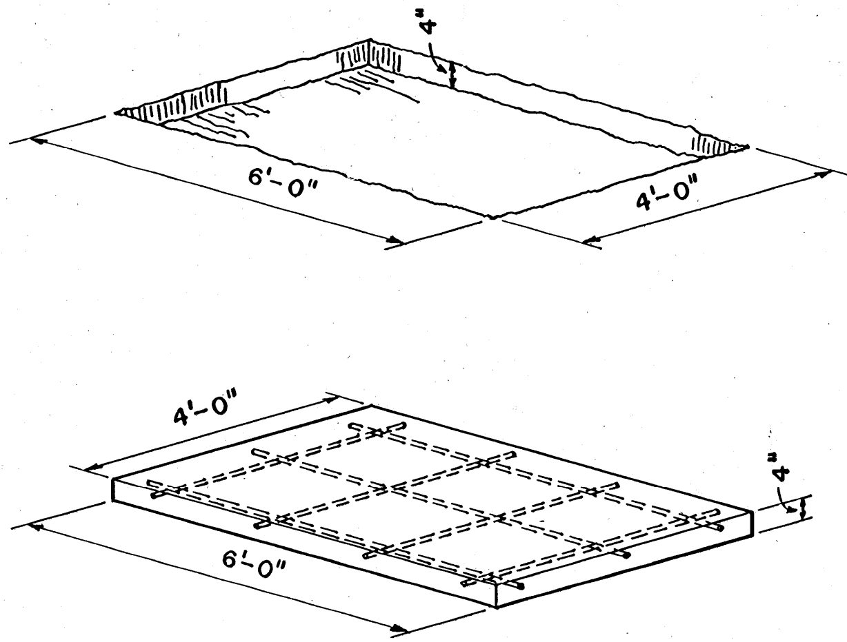
REINFORCED CONCRETE SLAB
