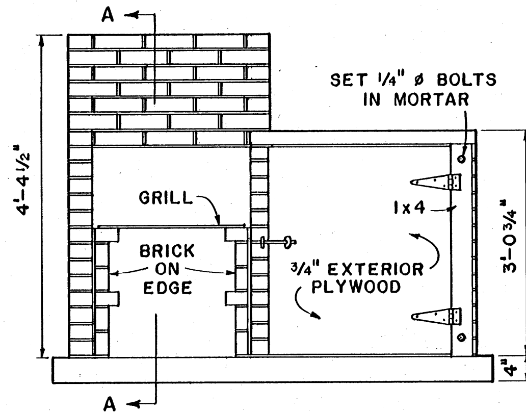
FRONT ELEVATION
