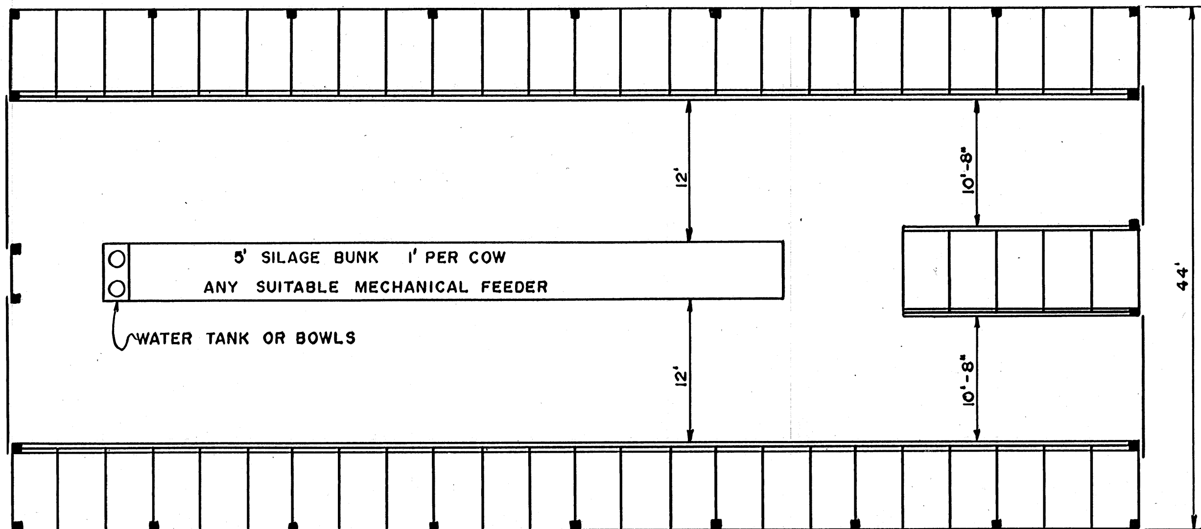
44' BARN FOR TWO ROWS FREE STALLS, CENTER FEEDER
