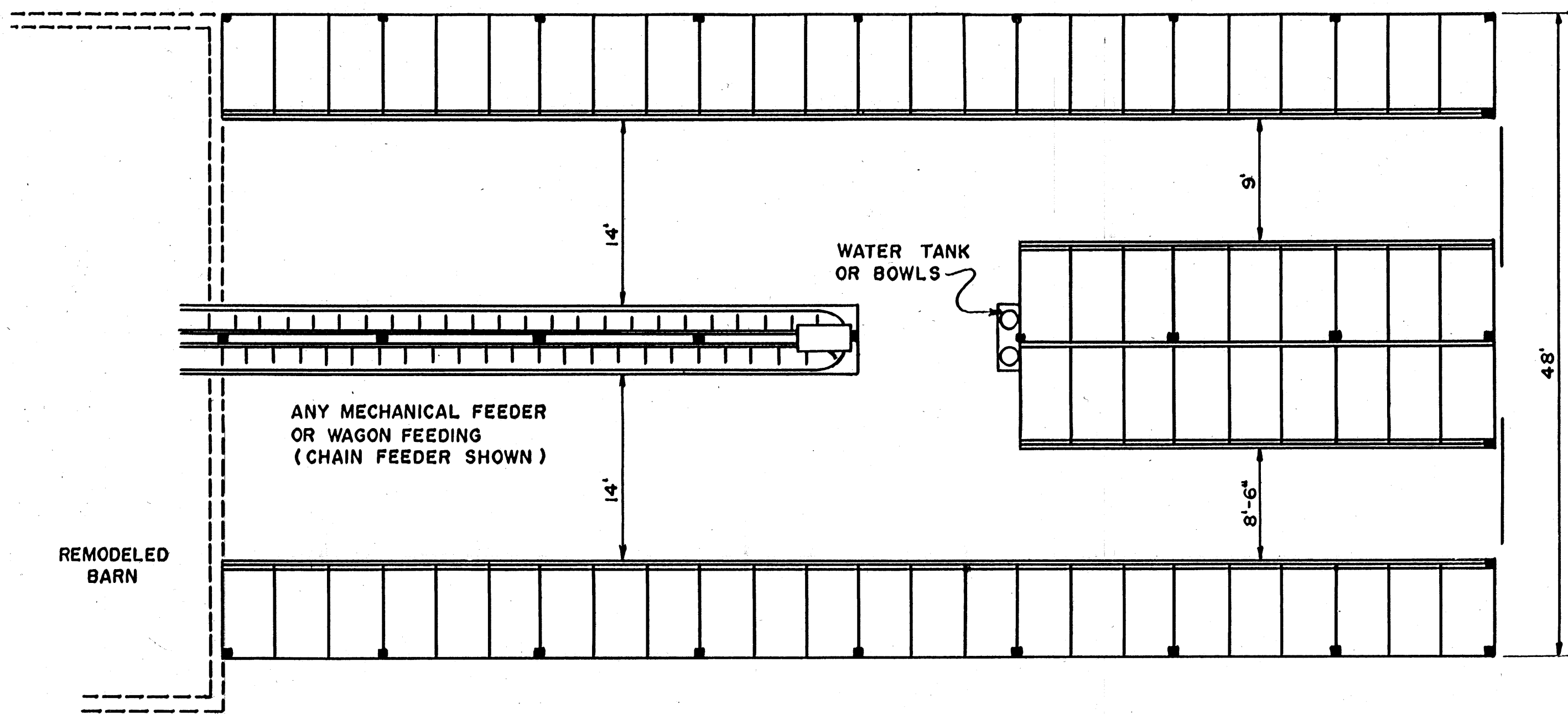
48' BARN FOR FOUR ROWS OF FREE STALLS CENTER FEEDER IF DESIRED
