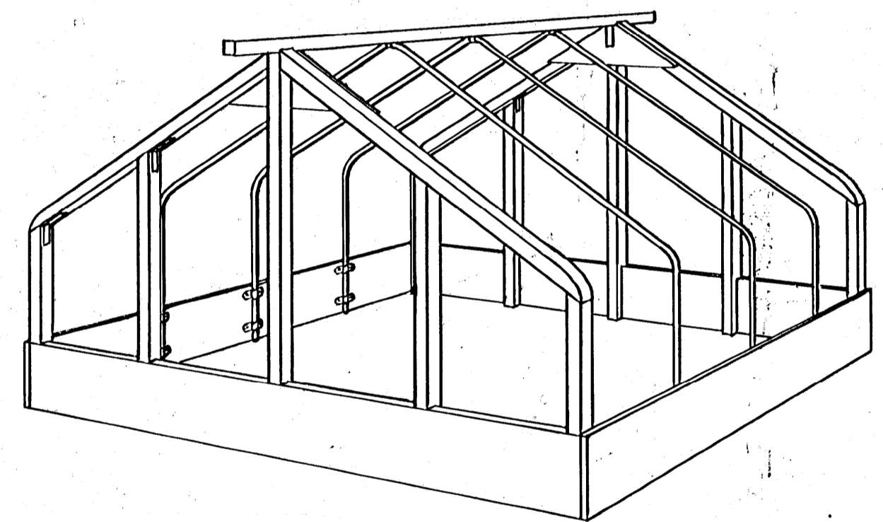
PERSPECTIVE VIEW FRAMING ONLY
