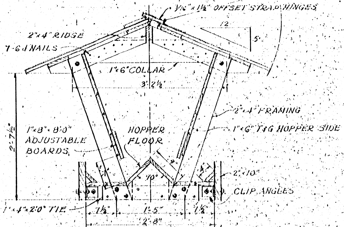
DETAIL OF INTERMEDIATE FRAMING SCALE: 1/4"=1'-0"
