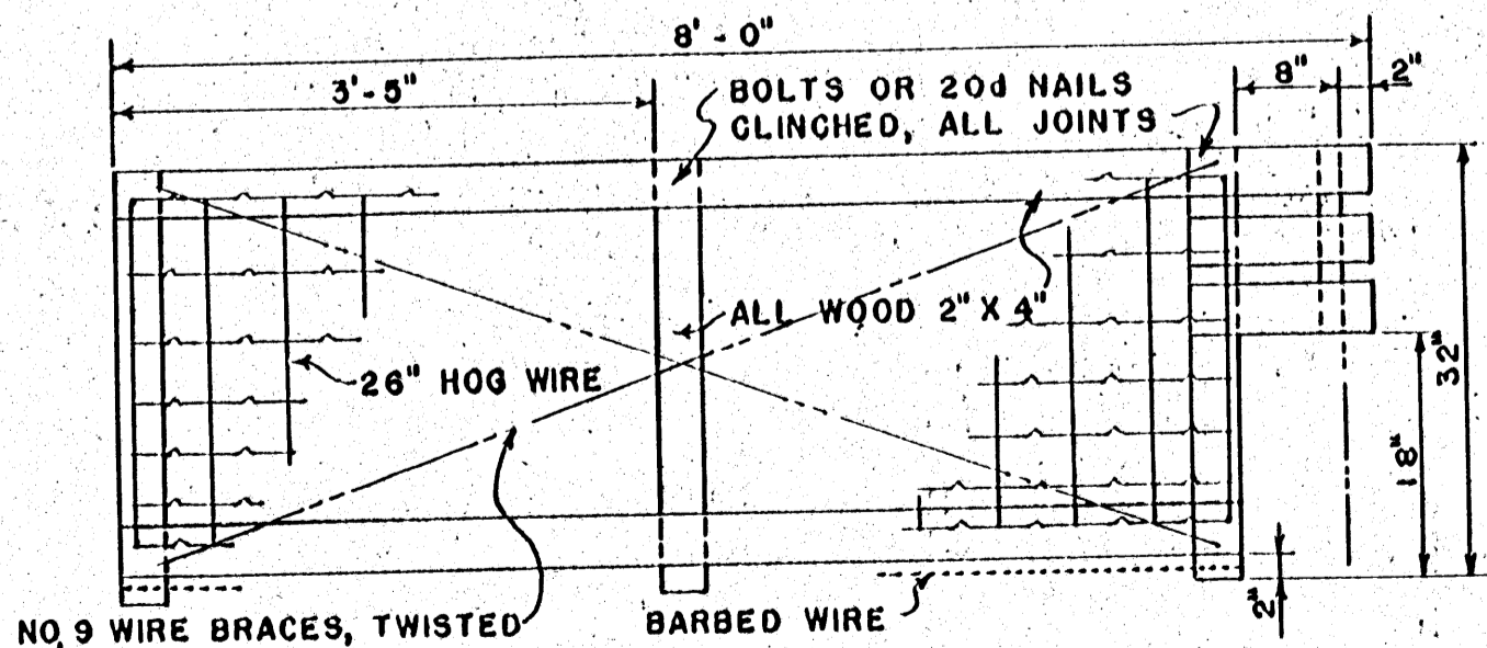
ALTERNATE PANEL CONSTRUCTION SUITABLE FOR HOT CLIMATES SCALE 3/4" = 1'-0"
