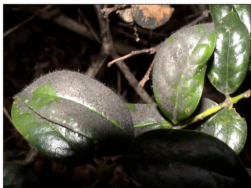
Figure 2. Vigorously growing sooty mold on holly. Note the sooty mold fungi are producing stalks (conidiophores) to launch their spores into the air.
