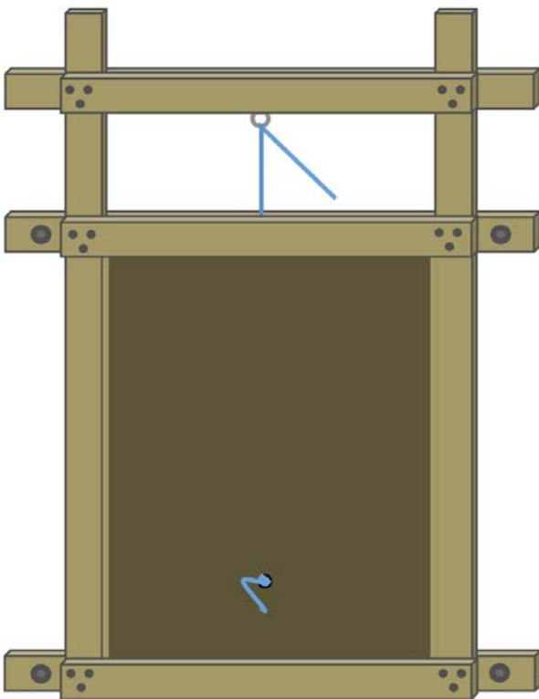
Figure 4. The “poor man’s” wooden drop door.
