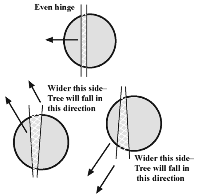
Three different hinges and how they affect the direction of the fall
