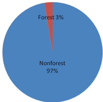
Total Area (452,084 acres; 8,628.8 acres in the USDA Conservation Reserve Program)
