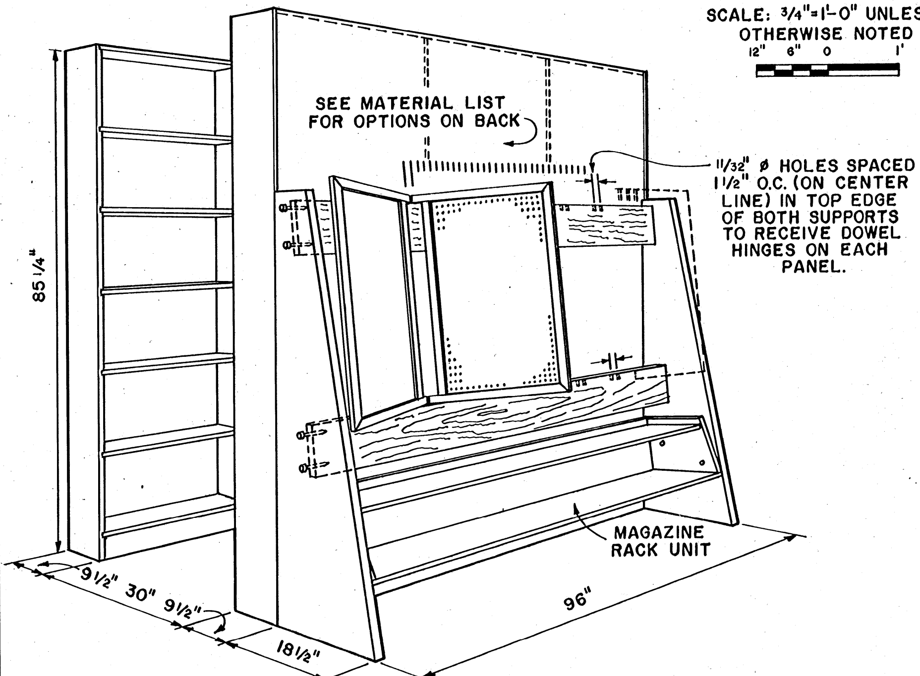
OVERALL VIEW SHOWING SPACE REQUIREMENTS NO SCALE
