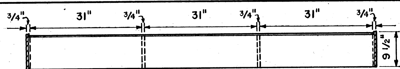
TOP VIEW
