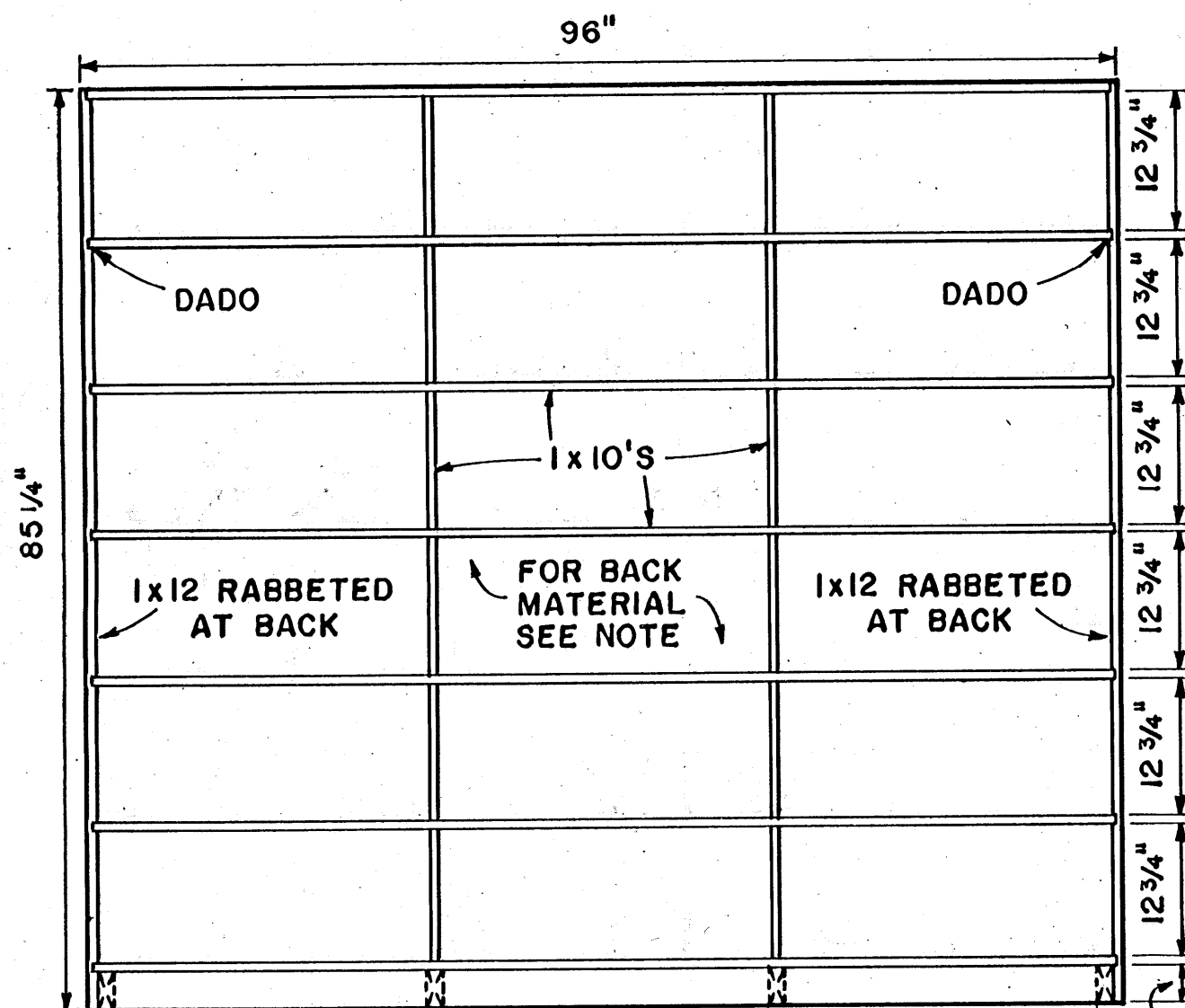
FRONT VIEW
