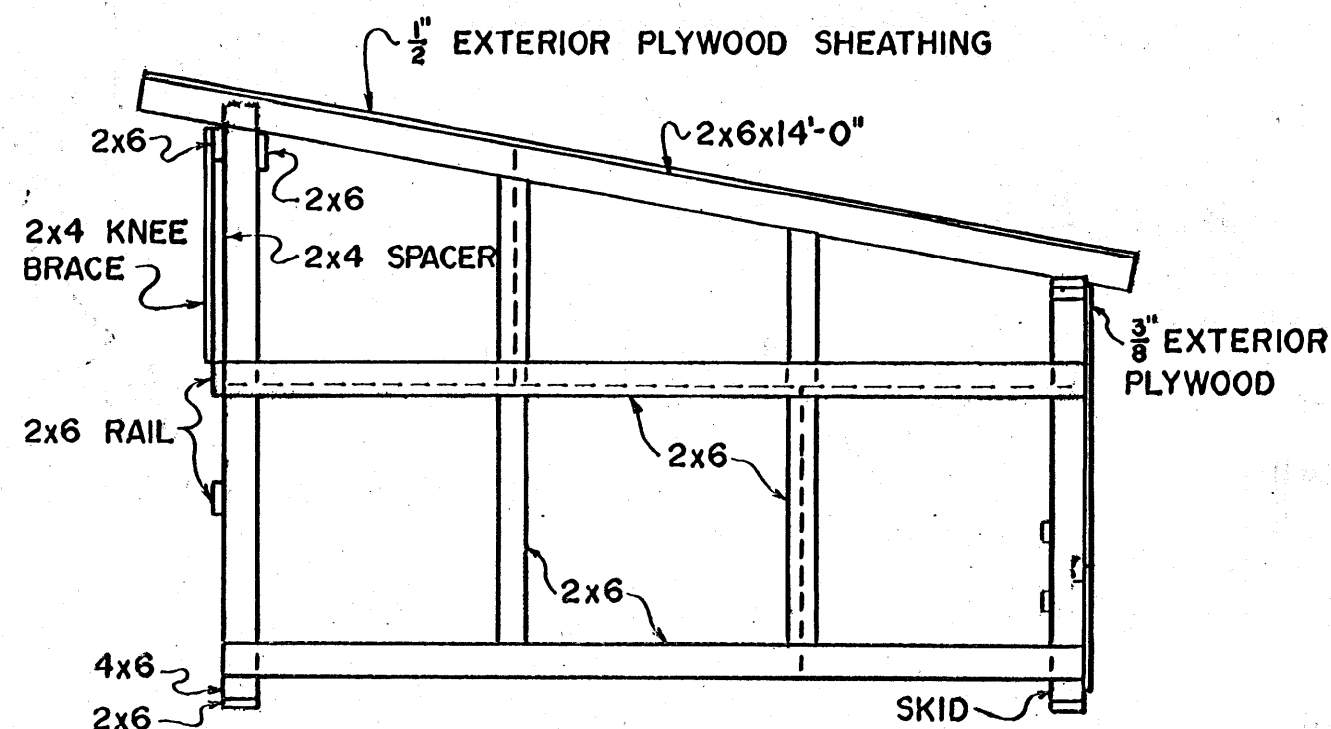
END FRAMING
