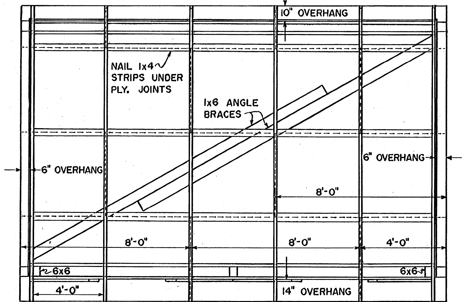
ROOF FRAMING
