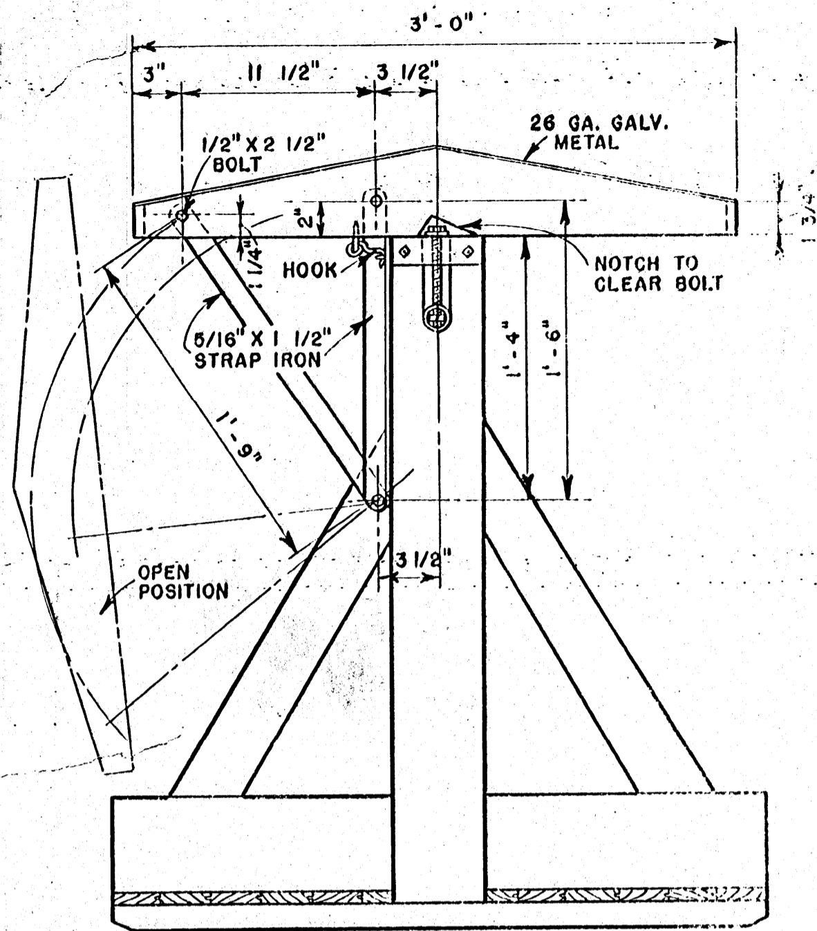
COVER DETAIL SHOWING FIT SCALE: 1 1/2" = 1'-0"
