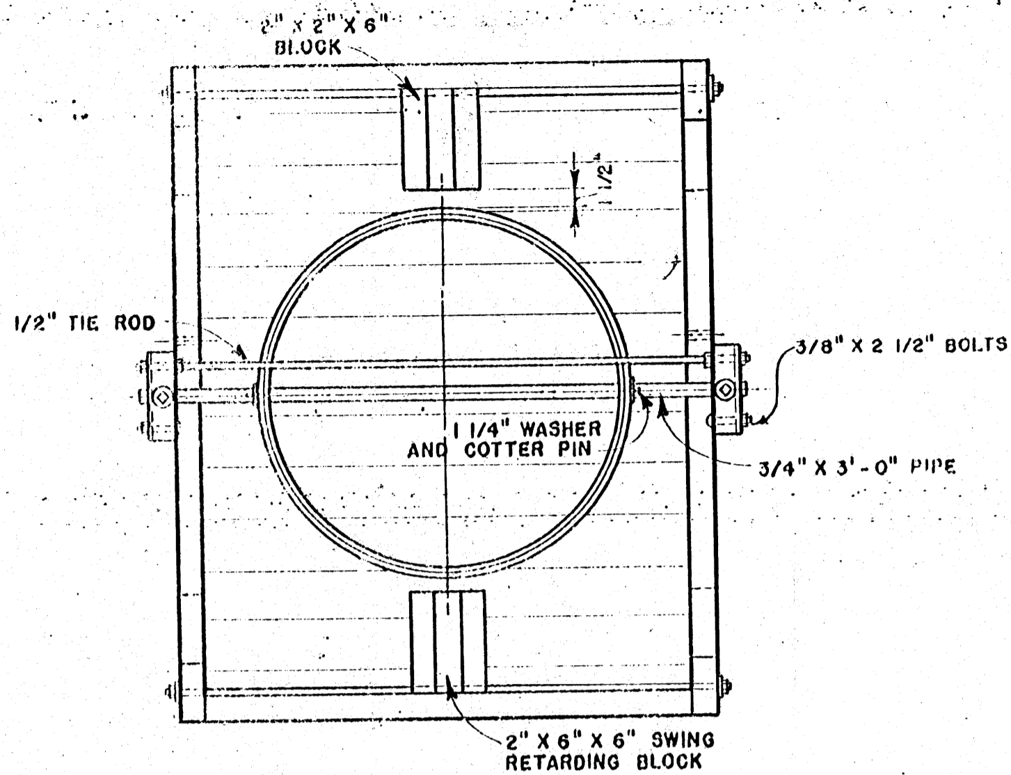
PLAN COVER NOT SHOWN
