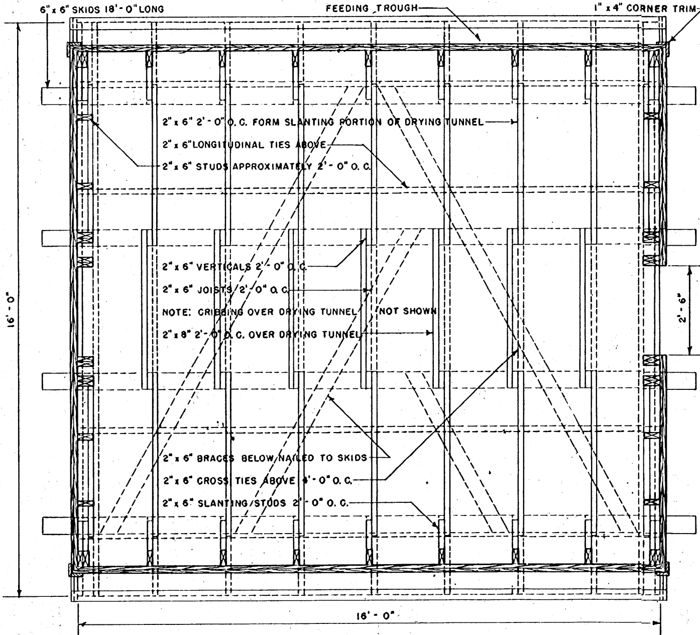
PLAN
