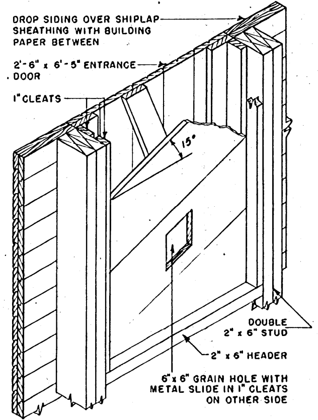
DETAIL AT ENTRANCE DOOR NOT TO SCALE
