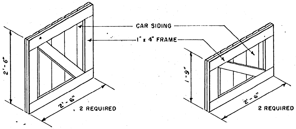
FILLING DOOR NOT TO SCALE
