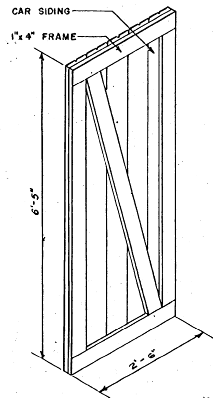
ENTRANCE DOOR NOT TO SCALE
