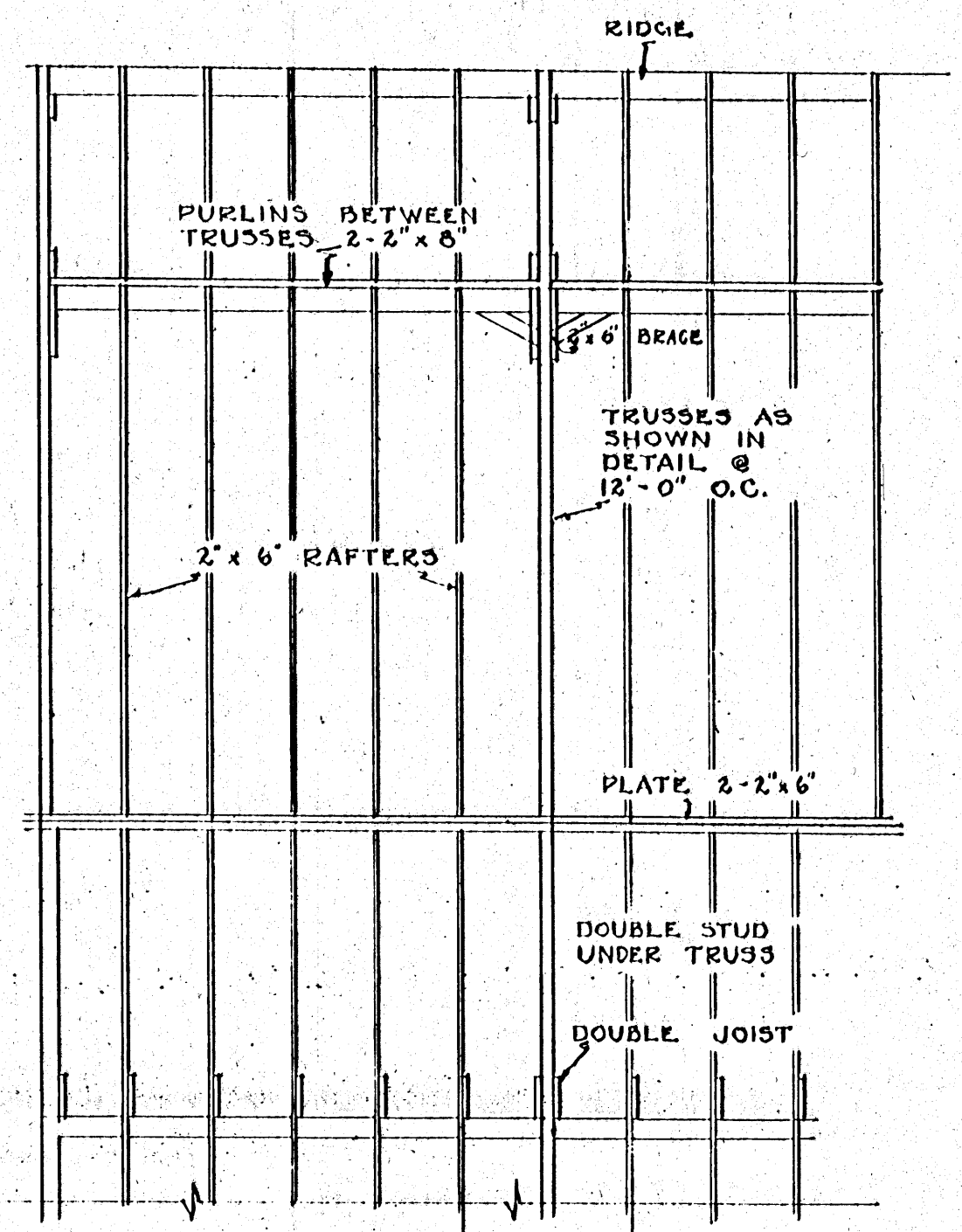
PART SIDE ELEVATION OF FRAMING SCALE: 1/4" = 1'-0"
